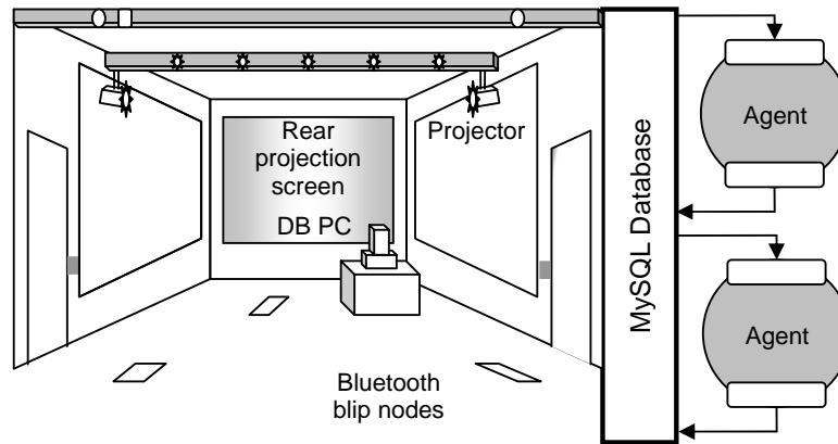
Figure 4. The curious research space agent society and its environment.
