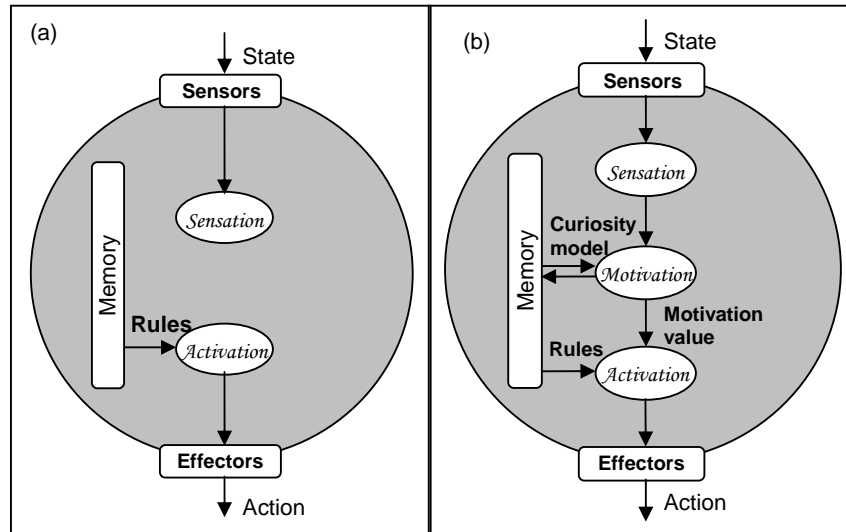
Figure 5. (a) Reflex agents and (b) motivated agents.
