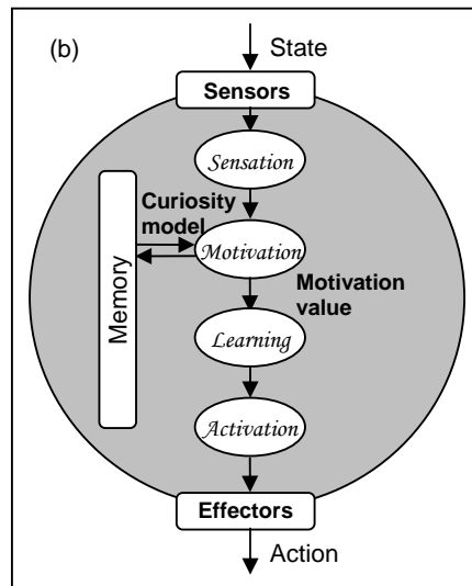
Figure 2. Motivated reinforcement learning agent model used to control the curious information display.
